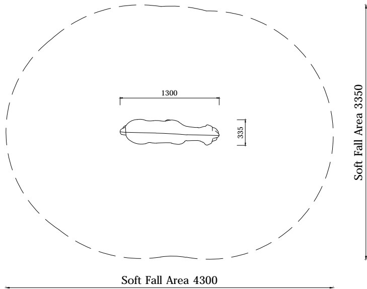
PLAN LAYOUT
